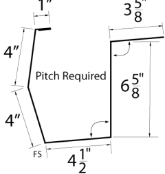
Pre Hung Gutter
