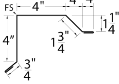
Gable
