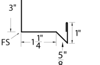
Inside Angle 2
