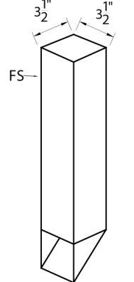
Down Spout Elbow 95
