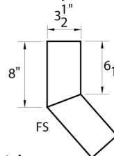
Down Spout Elbow 45
