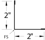
Outside Angle 2
