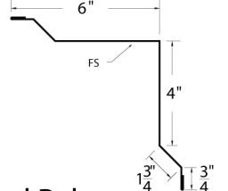
Sculptured Rake End Cap
