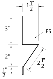
Base Guard
