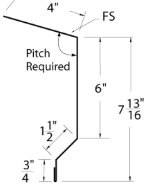
Fascia
