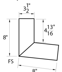
Down Spout Elbow 95
