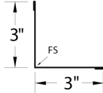
Inside Angle 3
