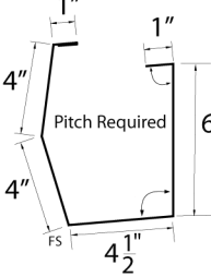
Gutter Support Strap
