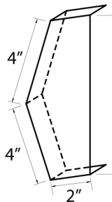
Sculptured Rake End Cap
