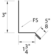
Base Drip
