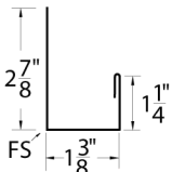
J Trim
