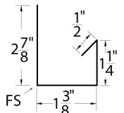
Rake and Corner
